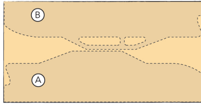
(2) - \frac{3}{4} " x 49" x 97" MDF, #37461
